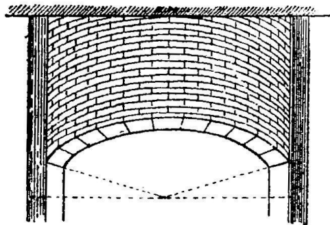
Fig. 3.—Projection horizontale.
