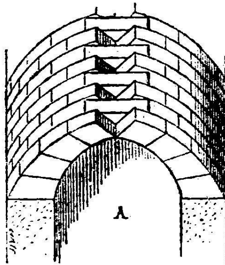
Fig. 1.—Projection horizontale.
