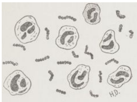
Fig. 14. — Streptococcus pyogenes .
