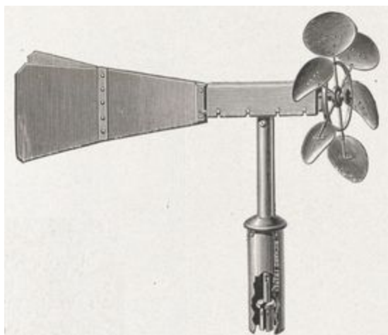
Fig. 50 bis. — Moulinet Richard.
