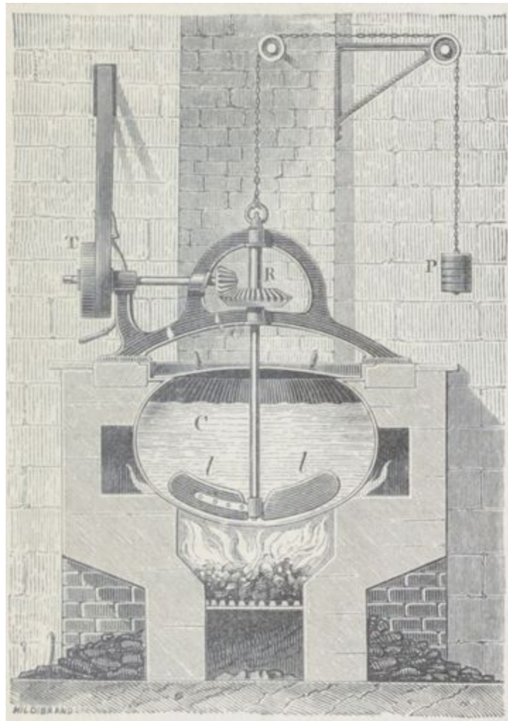
Foyer industriel.
