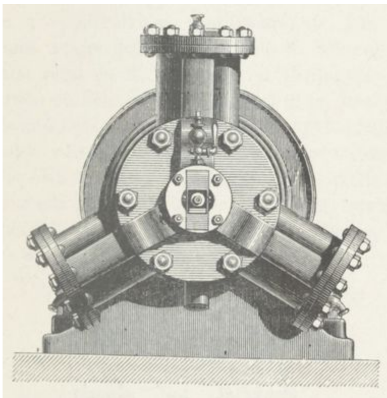
Fig. 66. — Machine Broterhood.
