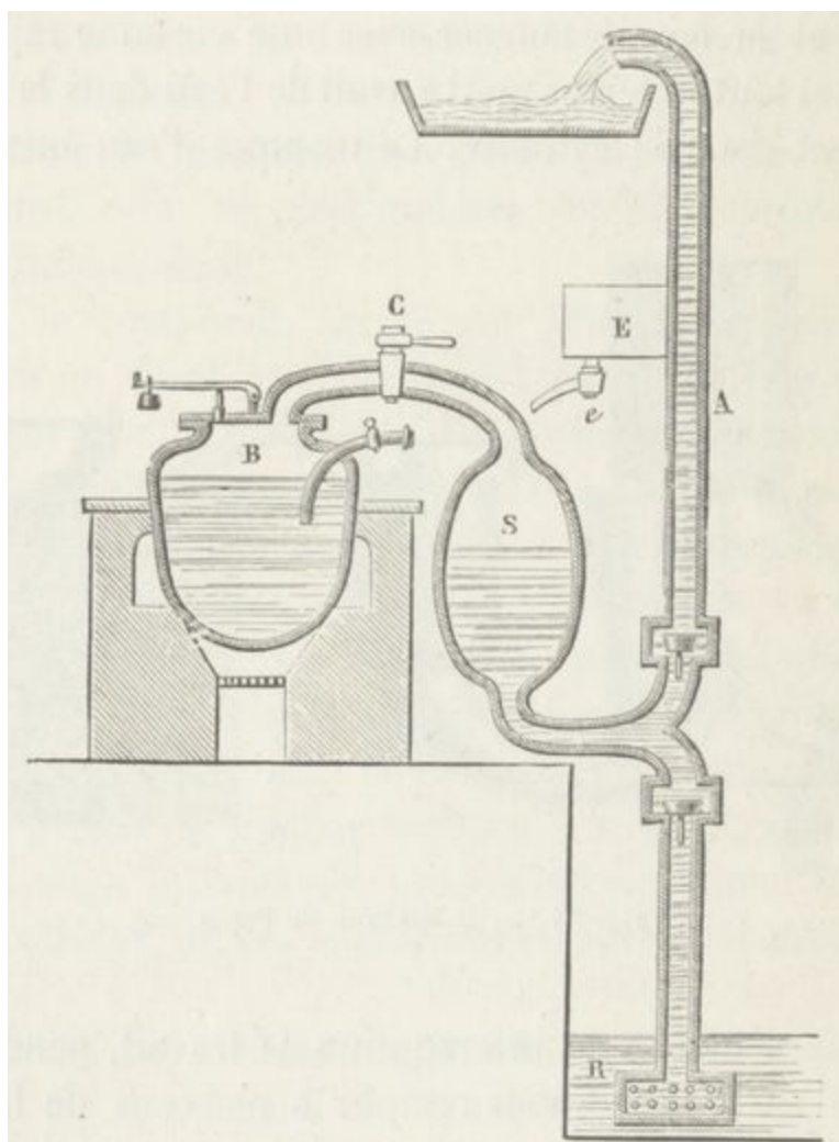
Fig. 39. — Machine de Savery.
