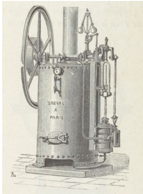
Fig. 62. — Machine Bréval.
