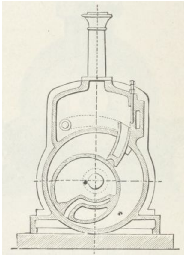
Fig. 67. — Machine rotative Uhler.
