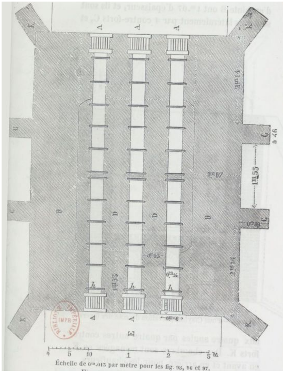
Fig. 95. — Four Clayton (plan).
