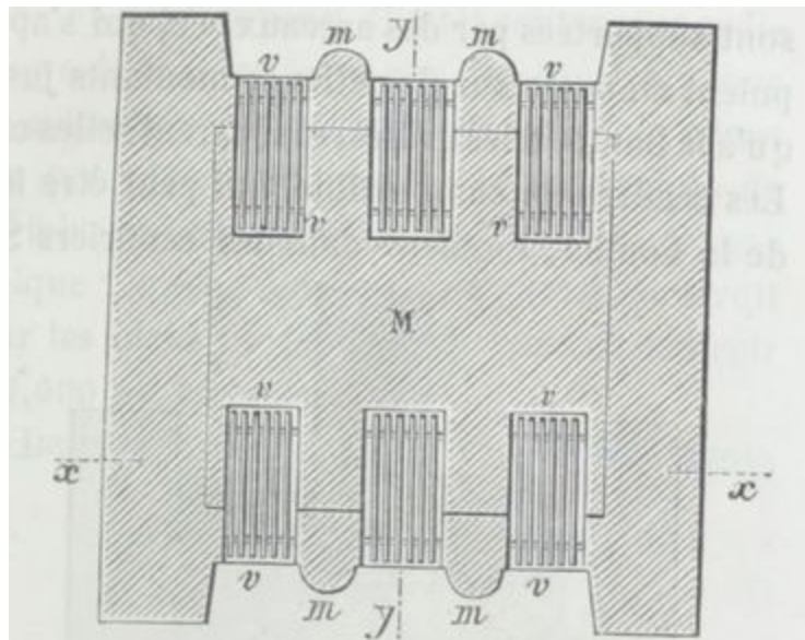
Fig. 90. — Four de Saint Meuge (plan).
