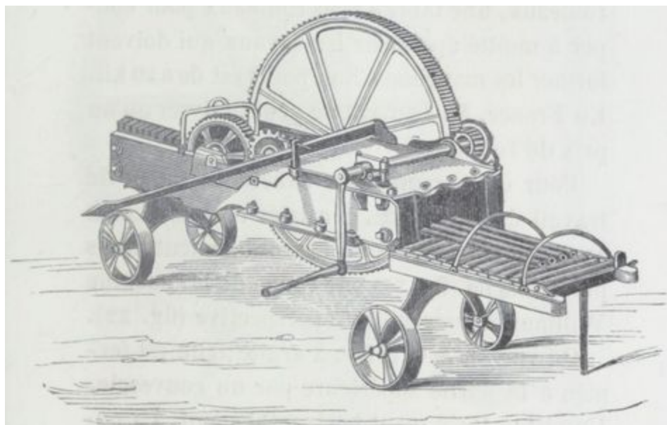
Fig. 32. — Machine de Williams.
