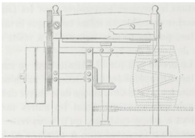
Fig. 51. — Projection verticale de la machine Champion.
