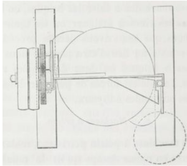
Fig. 52. — Projection horizontale de la machine Champion.
