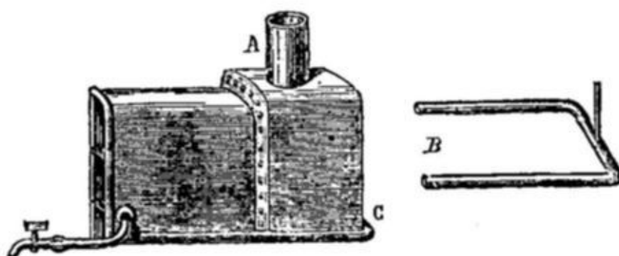
Fig. 2.—Thermosiphon. [2]
