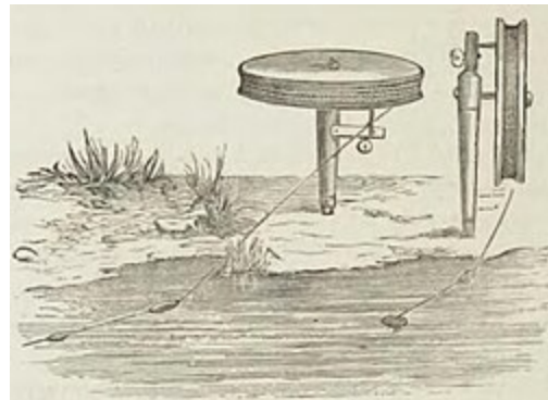
FIG. 118. — Grelot horizontal. FIG. 119. — Grelot vertical.
