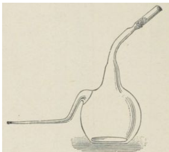
FIG. 14. — Ballon-pipette Chamberland.
