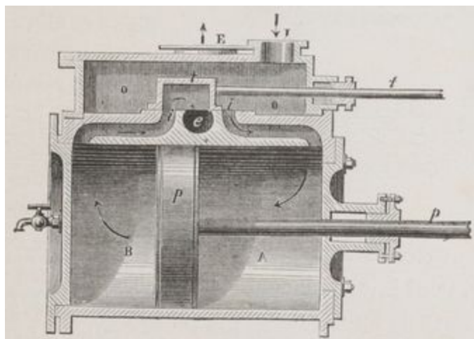
TIROIR (seconde position).
